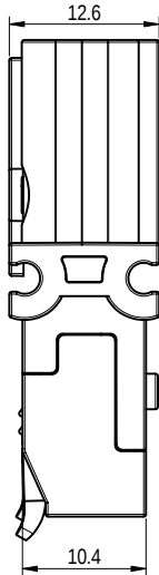
DGBSC-PG01M&F/4-00ZH-Lock_hook Scale 1: 1
